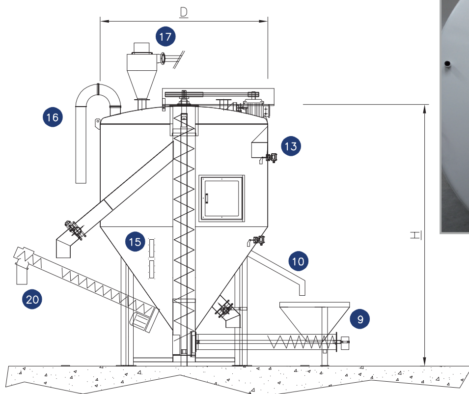
MISURE STANDARD MESCOLATORI MOD. CF - STANDARD MIXING MEASURES MOD. CF
